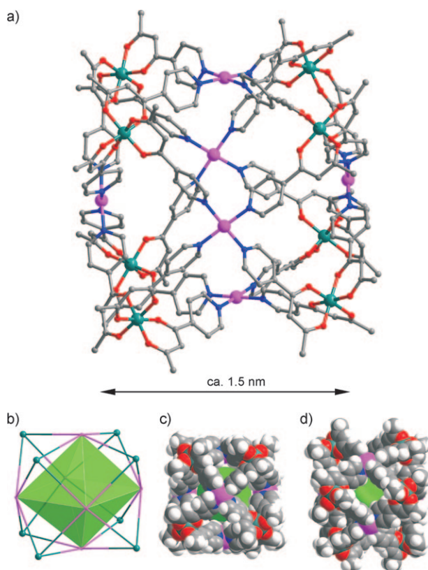
Figure 2. a) Molecular structure of the cation (\Lambda\Lambda\Lambda\Lambda\Lambda\Lambda\Lambda\Lambda)-[\text{Pd}_6(\text{AlL}_3)_8]^{12+} in 2 , hydrogen atoms are omitted for clarity; b) the capped octahedral arrangement of \text{Pd}_6\text{Al}_8 core in [\text{Pd}_6(\text{AlL}_3)_8](\text{NO}_3)_{12} ( 2 ); c) perspective drawing of the cation [\text{Pd}_6(\text{AlL}_3)_8]^{12+} in space-filling mode; d) [\text{Pd}_6(\text{AlL}_3)_8]^{12+} viewed through the \text{Pd}_2\text{Al}_2 portal. The space inside the cage is shown as a dummy green ball with diameter of ca. 10 Å. Purple Pd; cyan Al; red O; blue N; gray C; white H.
